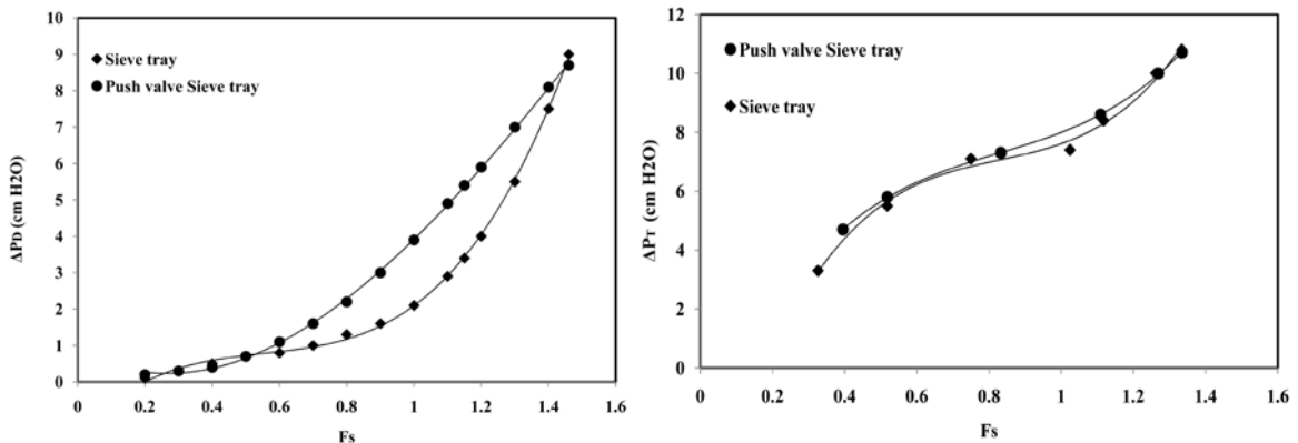
Figure 5. a) Dry pressure drop, b) Total pressure drop
