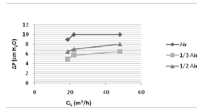
Fig. 6. performance characteristics
