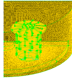
Fig. 2. Mesh configurations of the computational domain
