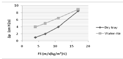
Fig.5. pressure drop for the centrifugal tray
